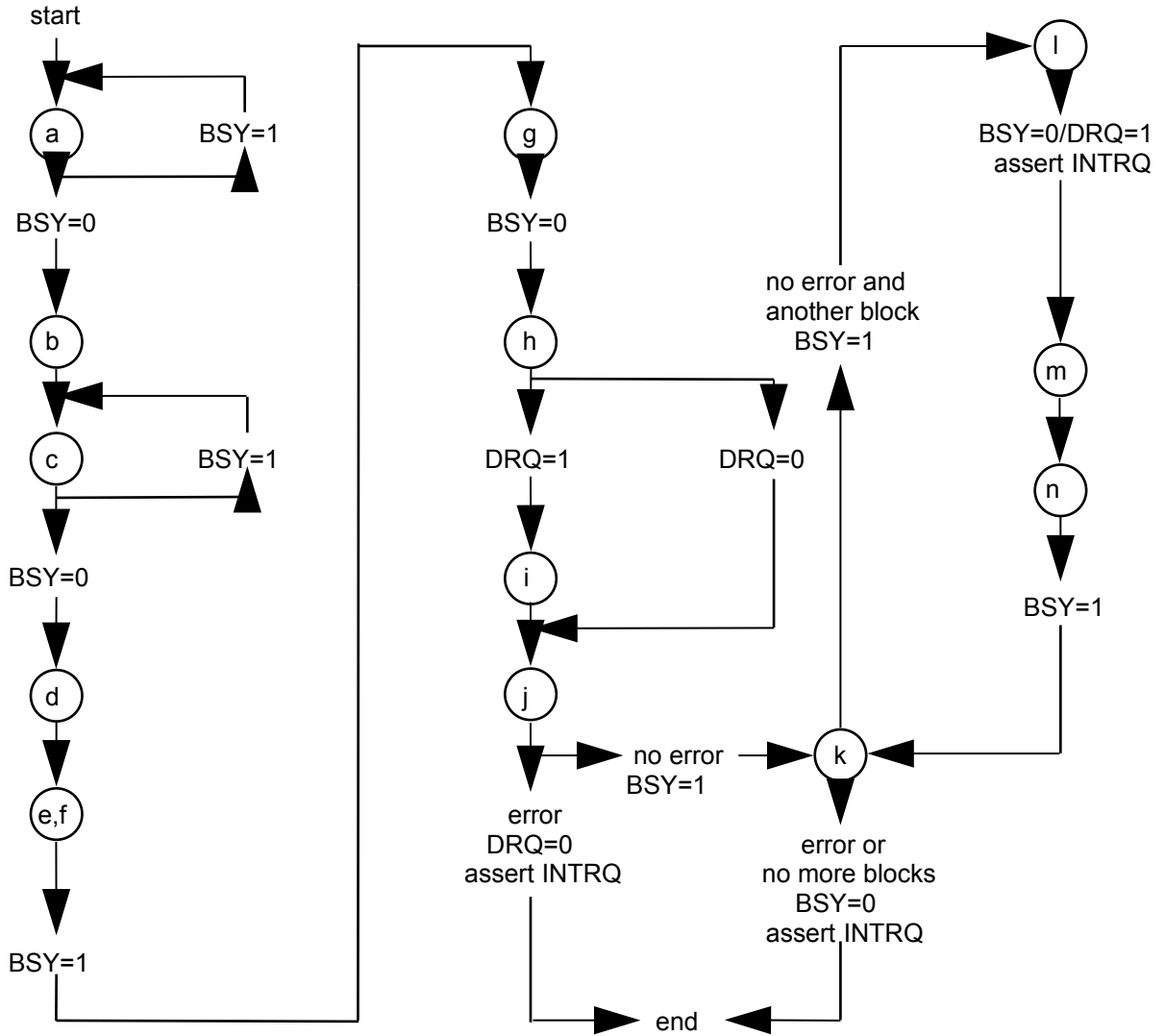
Figure 11 - PIO Data Transfer Out Diagram11
