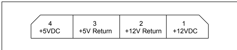
Figure 2 - Drive Side Connector Pin Numbering2
