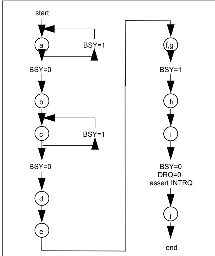
Figure 13 - DMA Data Transfer Diagram13
