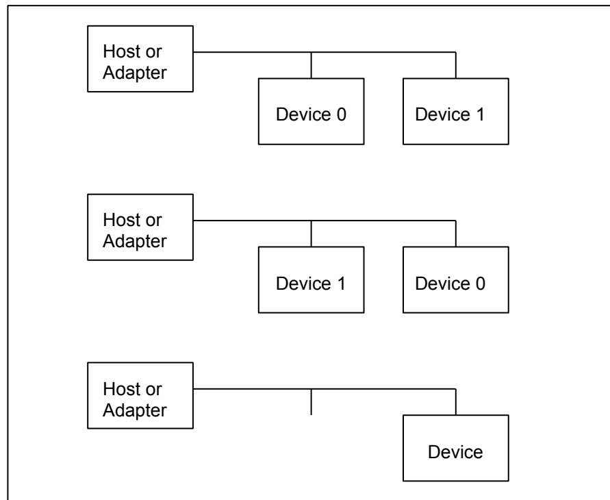
Figure 1- ATA Interface Cabling Diagram1
