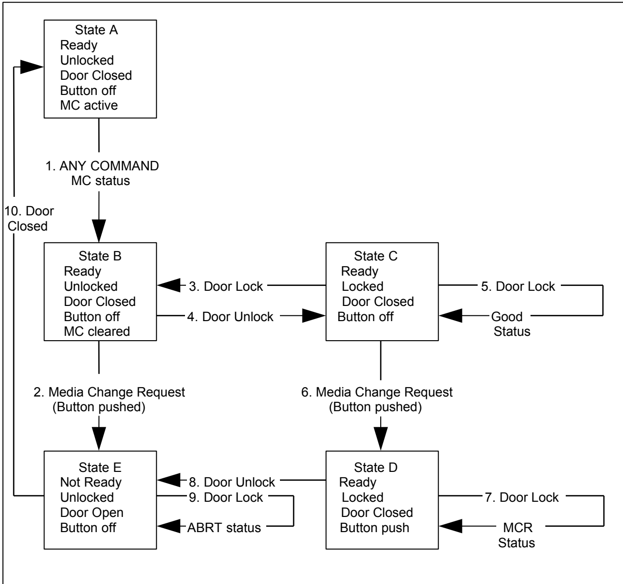
Figure 6 - Removable Modes6
