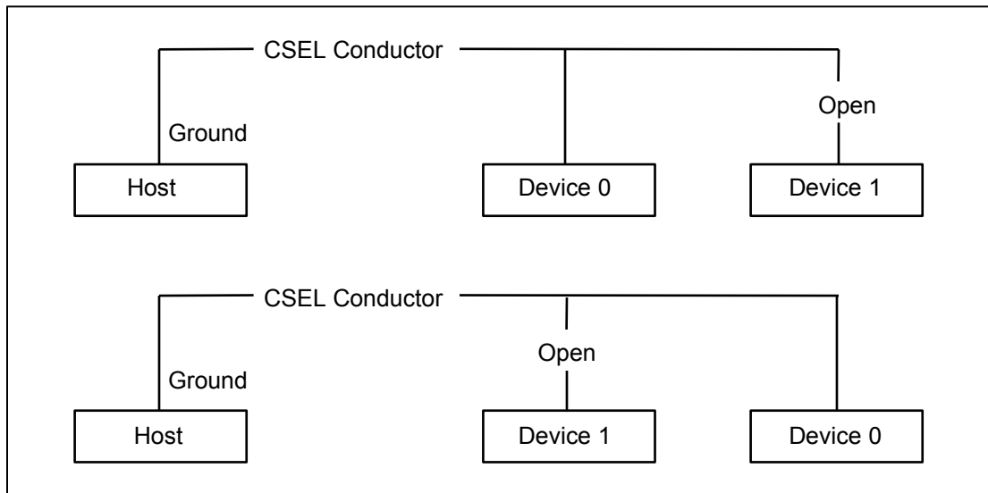
Figure 4 - Cable Select Example4
