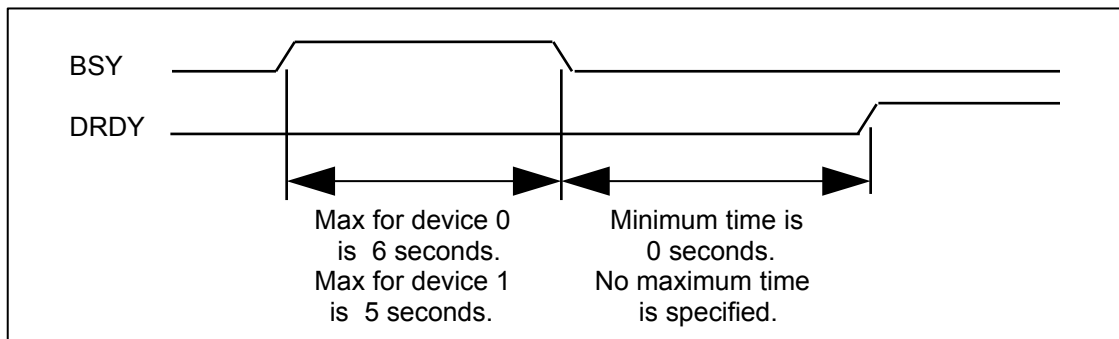
Figure 7 - BSY and DRDY timing for Diagnostic command7
