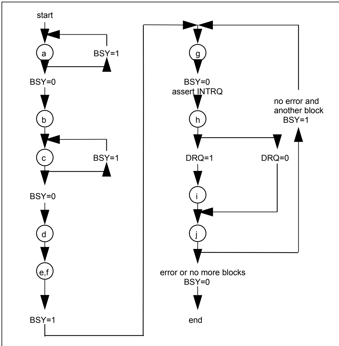
Figure 10 - PIO Data Transfer Diagram10
