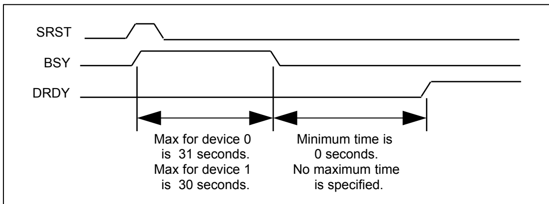
Figure 9 - BSY and DRDY timing for software reset9
