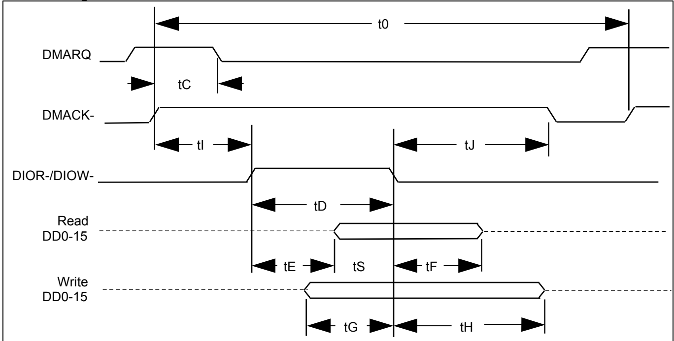
Figure 15 - Single Word DMA Data Transfer 15
