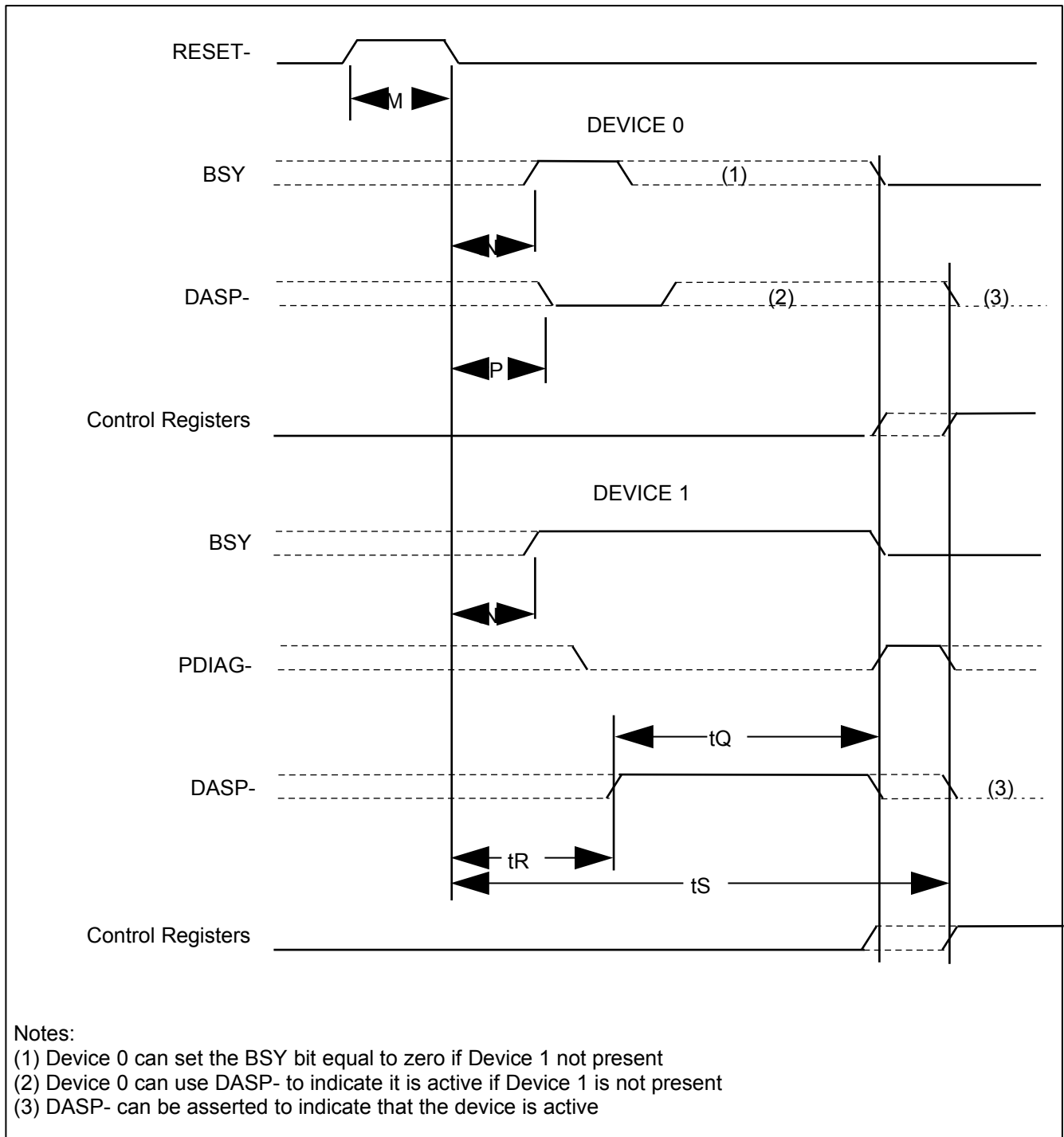
Figure 17 - Reset Sequence17
