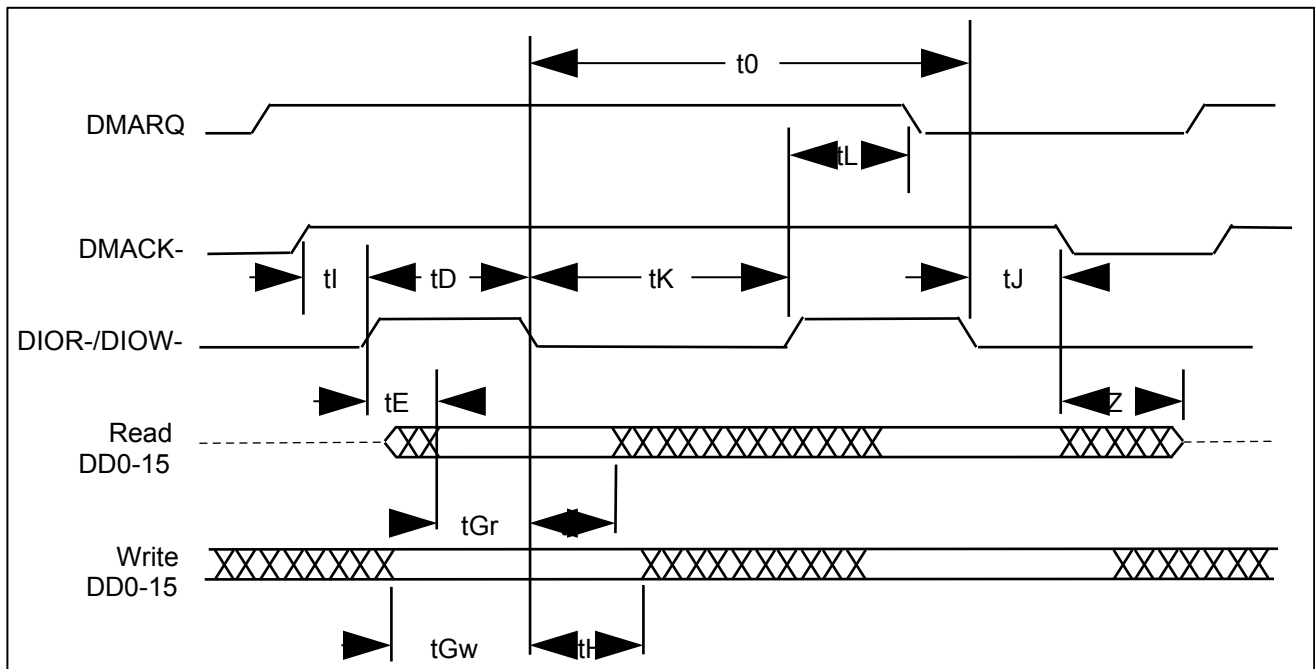
Figure 16 - Multiword DMA Data Transfer 16
